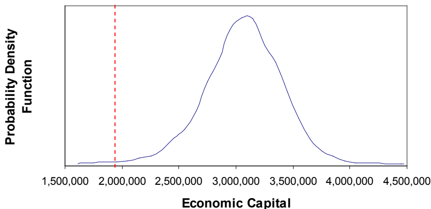
Figure 1: Distribution of Economic Capital
