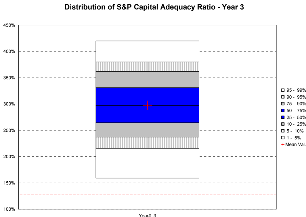
Figure 4: Distribution of Year 3 S&P CAR
