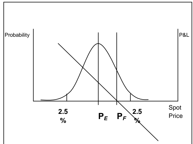
Figure 4. Payout function of available futures contract with management price expectations
